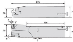
Right Hand Toolholder 69 391 458 10
