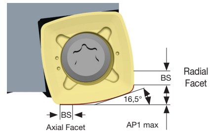
Perfect combination of round and square insert style.
